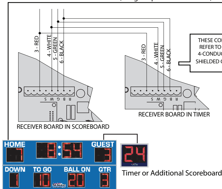
4 Conductor Twisted Data Cable (Length Specified w/ Order)
