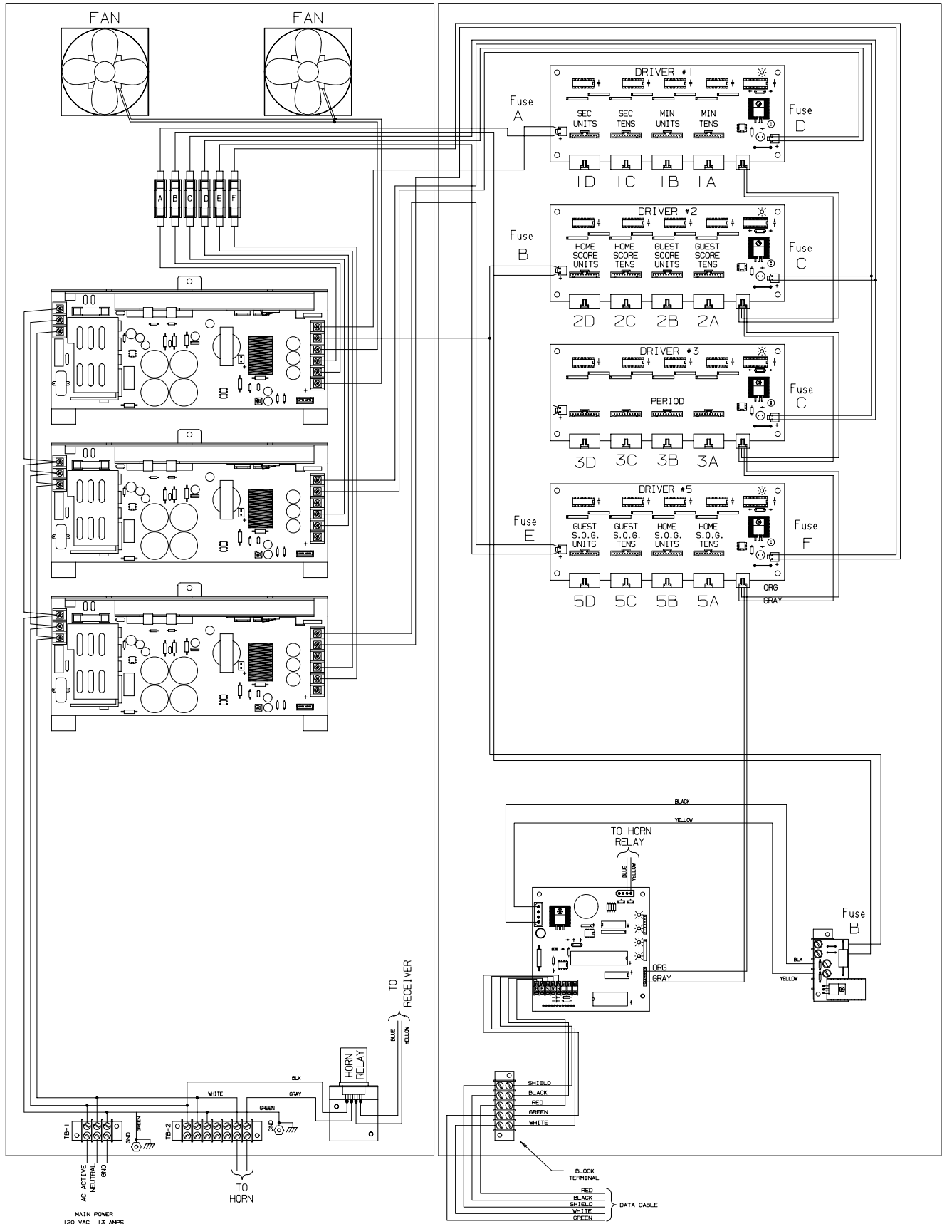
CONTROLLER ASSEMBLY
