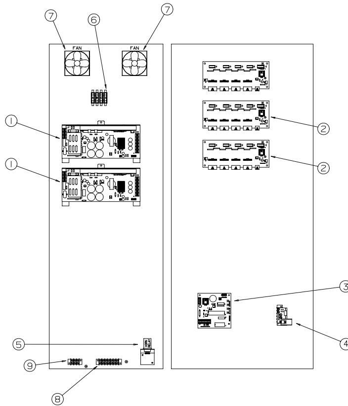
figure 2 CONTROLLER ASSEMBLY
