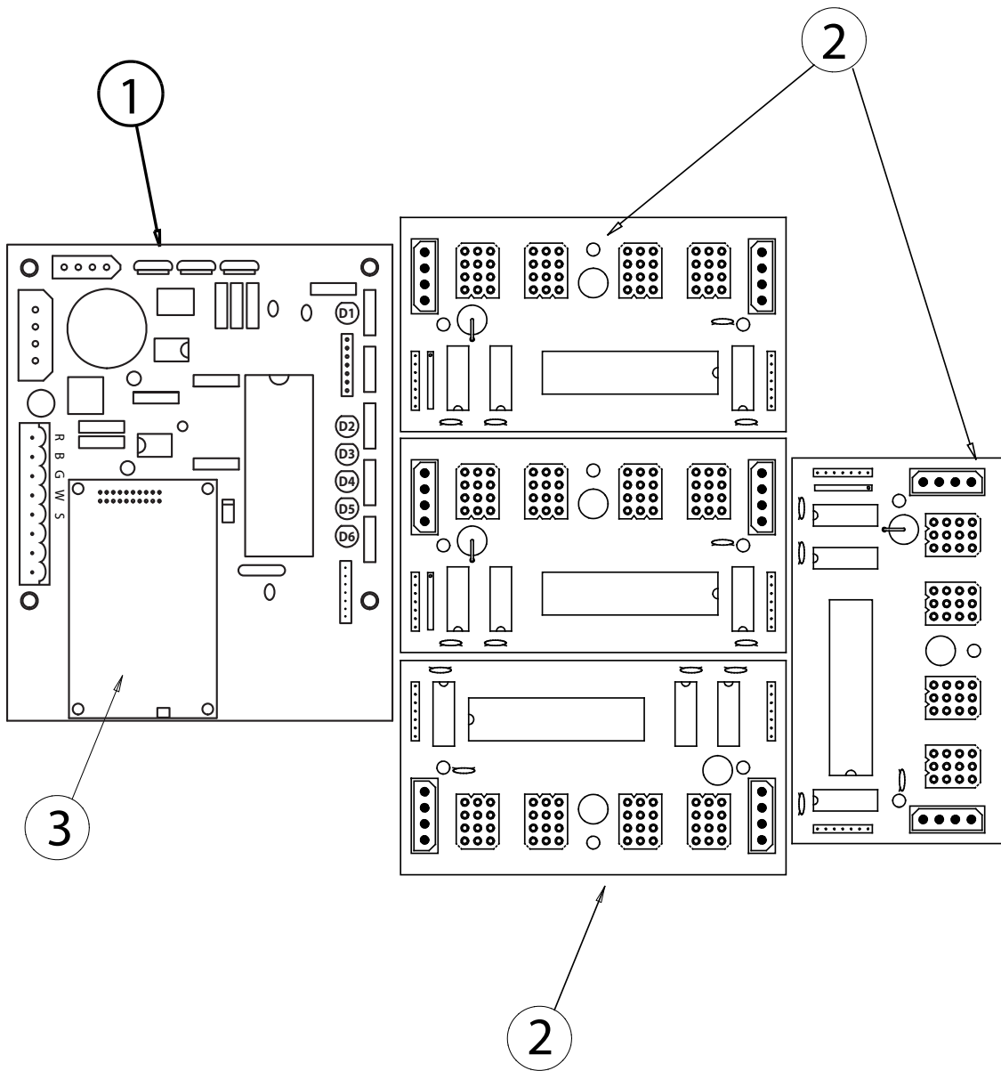
figure 2 CONTROLLER ASSEMBLY
