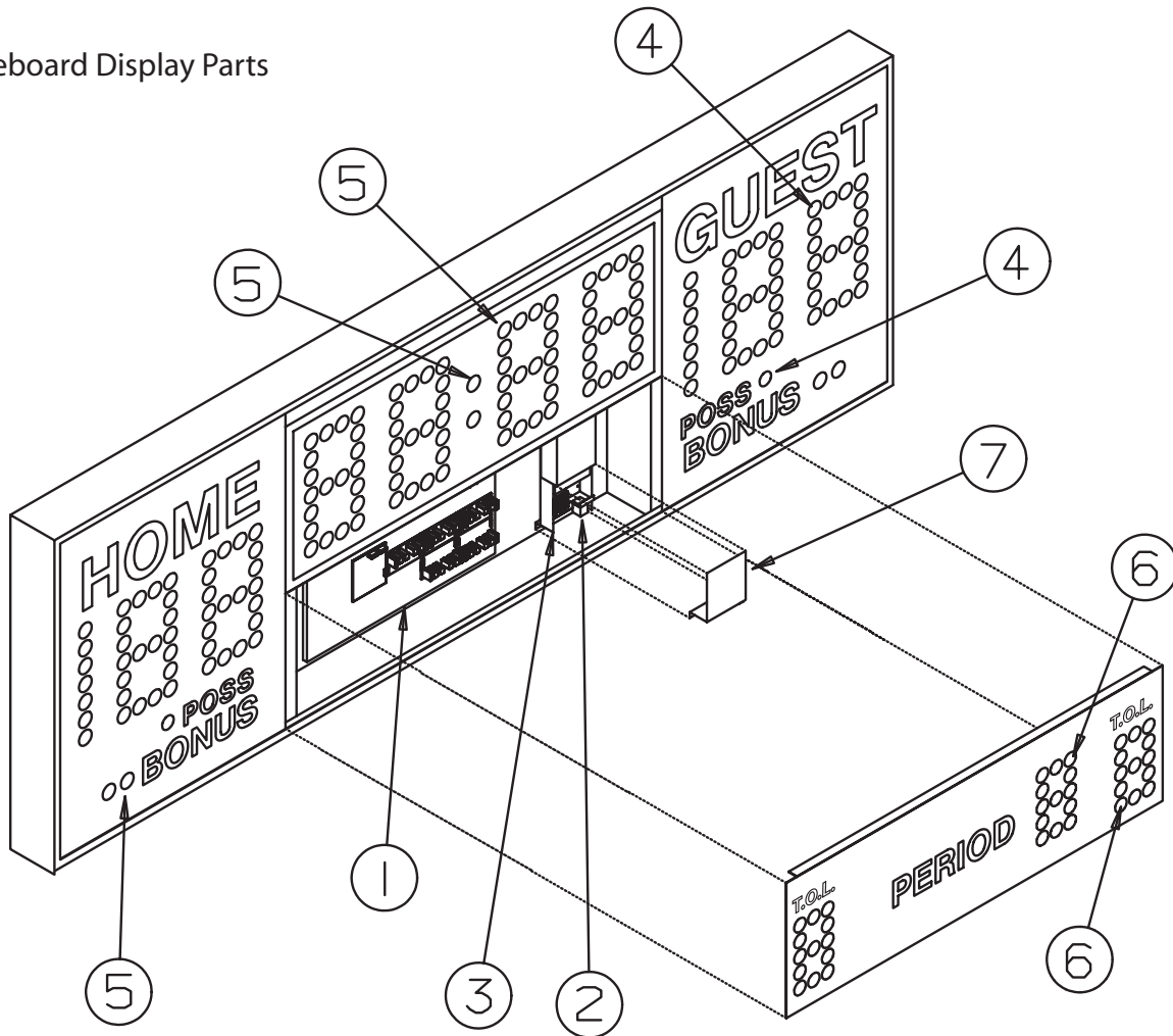
Figure 1 DISPLAY ASSEMBLY
