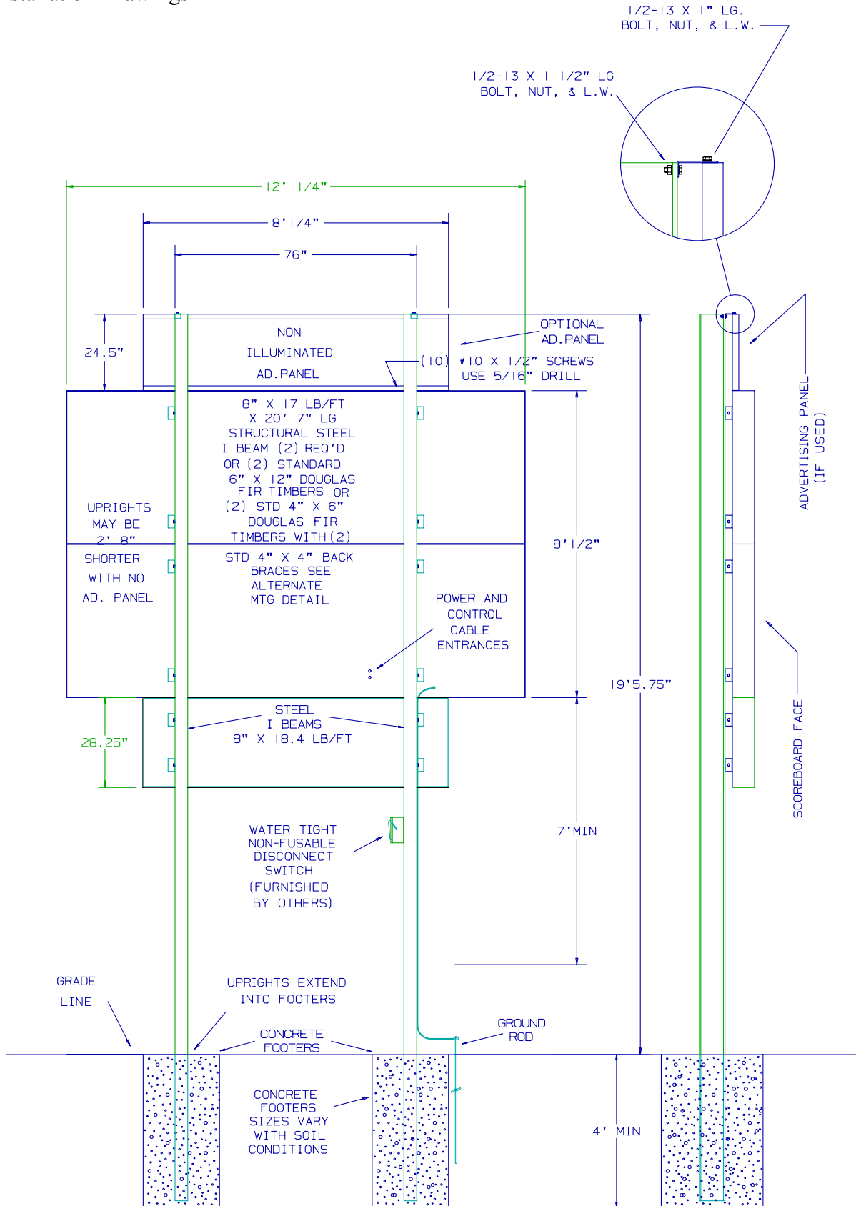
INSTALLATION DRAWING
