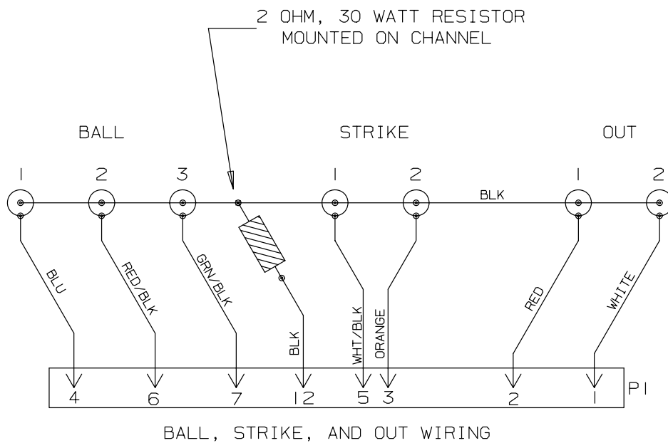
FIGUREGRAM WIRING
