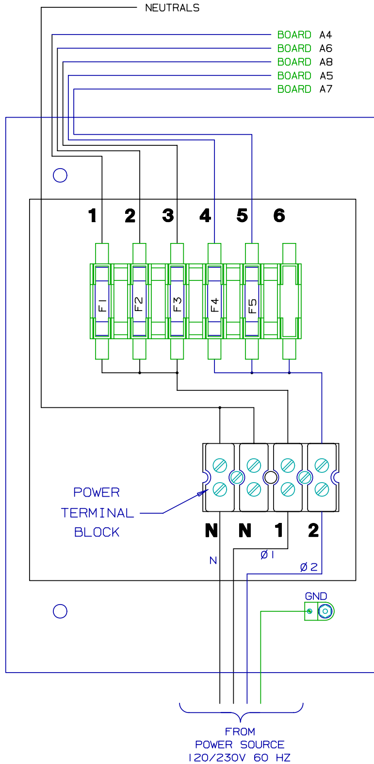
POWER WIRING
