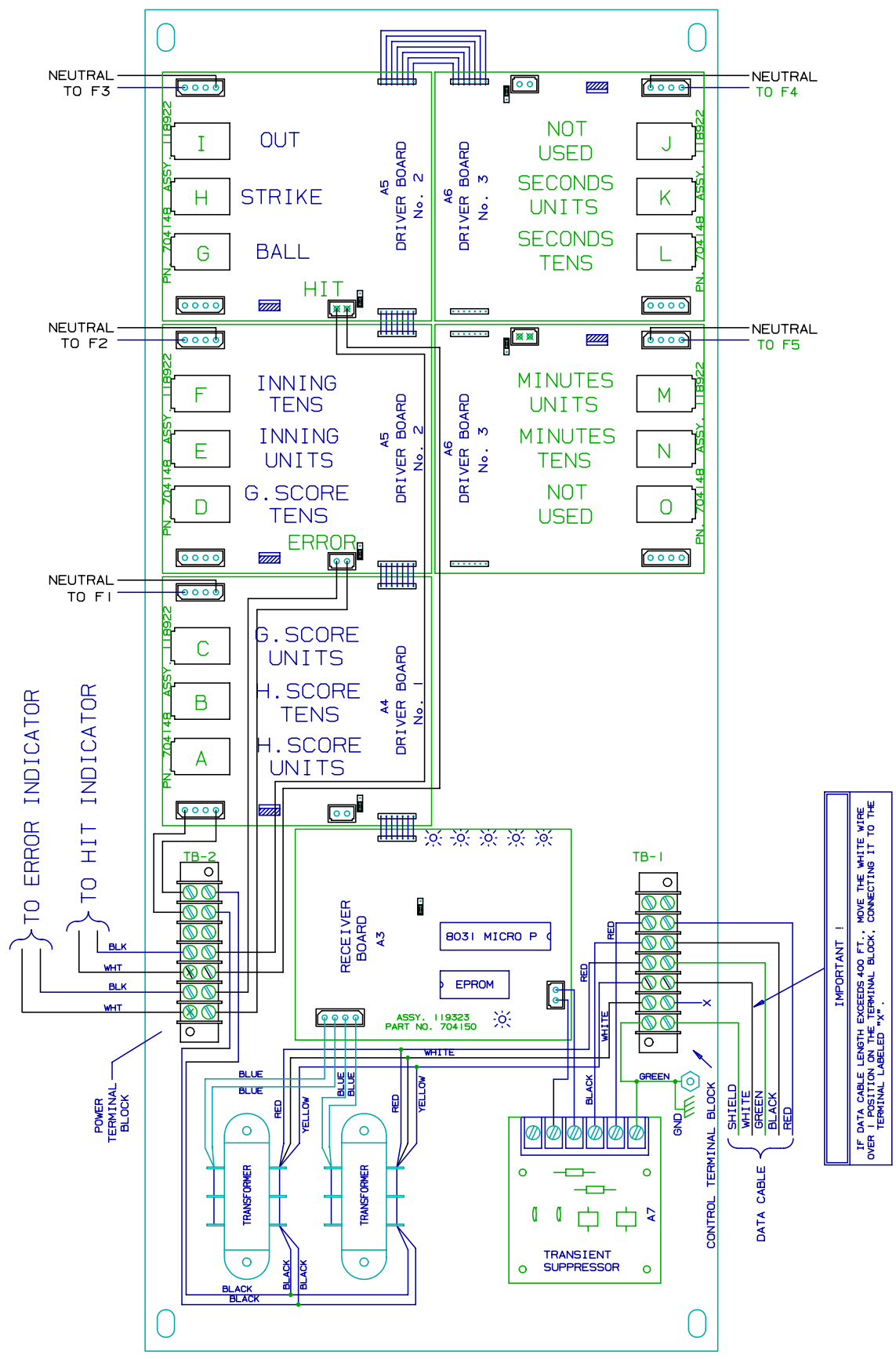
CONTROLLER ASSEMBLY
