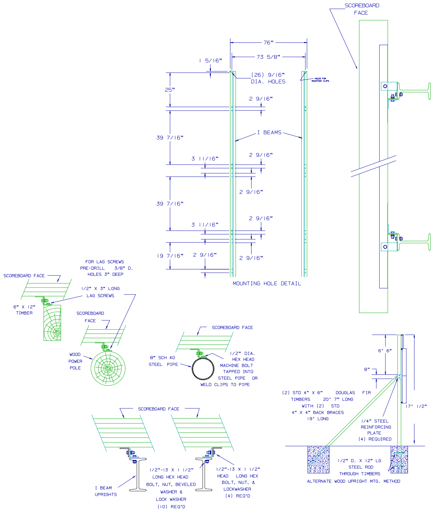
INSTALLATION DRAWING
