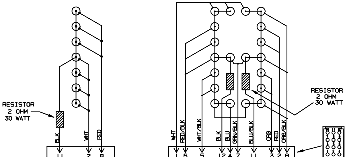
FIGUREGRAM WIRING 6.8 Jumper Location on 3 Position System
