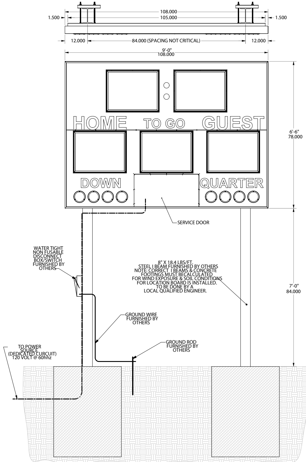
Figure 1: Site Elevation
